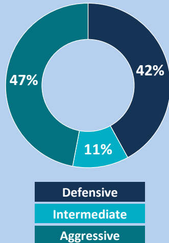
Bucket Allocation
